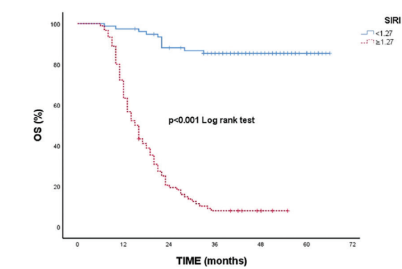
FIGURE 2: The Kaplan-Meier curves for OS according to SIRI levels. OS: Overall survival; SIRI: Systemic inflammation response index
