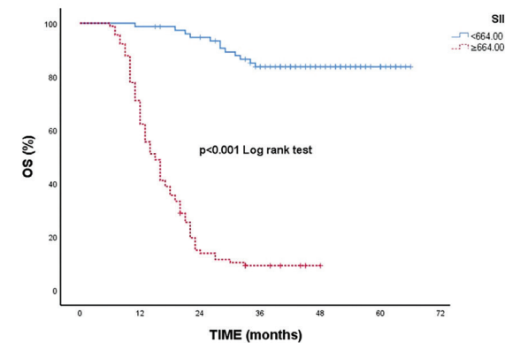
FIGURE 1: The Kaplan-Meier curves for OS according to SII levels. OS: Overall survival; SII: Systemic immune inflammation index
