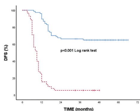
FIGURE 3: The Kaplan-Meier curves for DFS according to SII levels. DFS: Disease-free survival; SII: Systemic immune inflammation index
